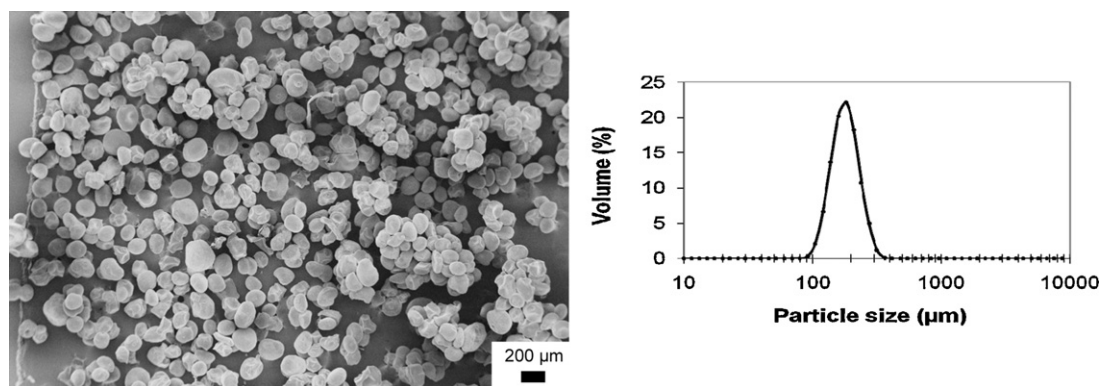
Fig. 6. SEM micrograph of LMAP microspheres loaded with erythrosin (ERY-LMAP) (initial magnification 200 \times ), and particle size distribution according to laser light scattering measurements.
