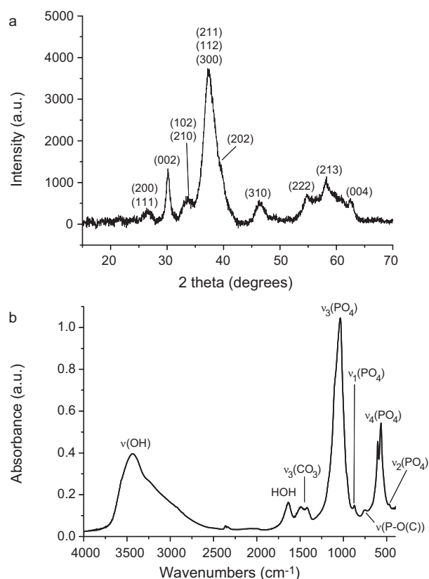
Fig. 1. (a) XRD patterns and (b) FTIR spectra for apatite colloidal nanoparticles.
